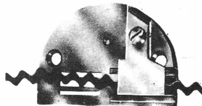
ADJUSTABLE RIC RAC OR LACE GUIDE, COMPLETE #S79
